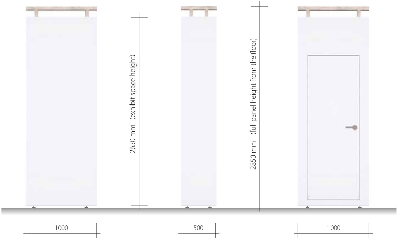
W1 wall panel
