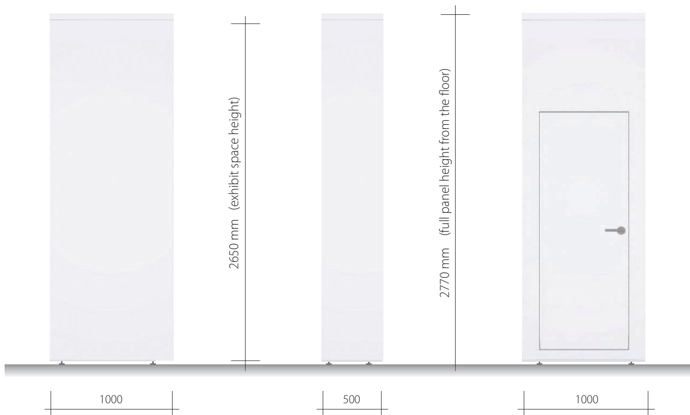
W1/265 wall panel
